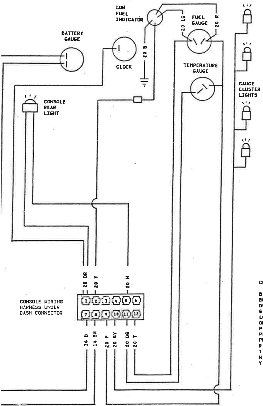
1967 CONSOLE WIRING MANUAL TRANSMISSION WITH CONSOLE GAUGES
