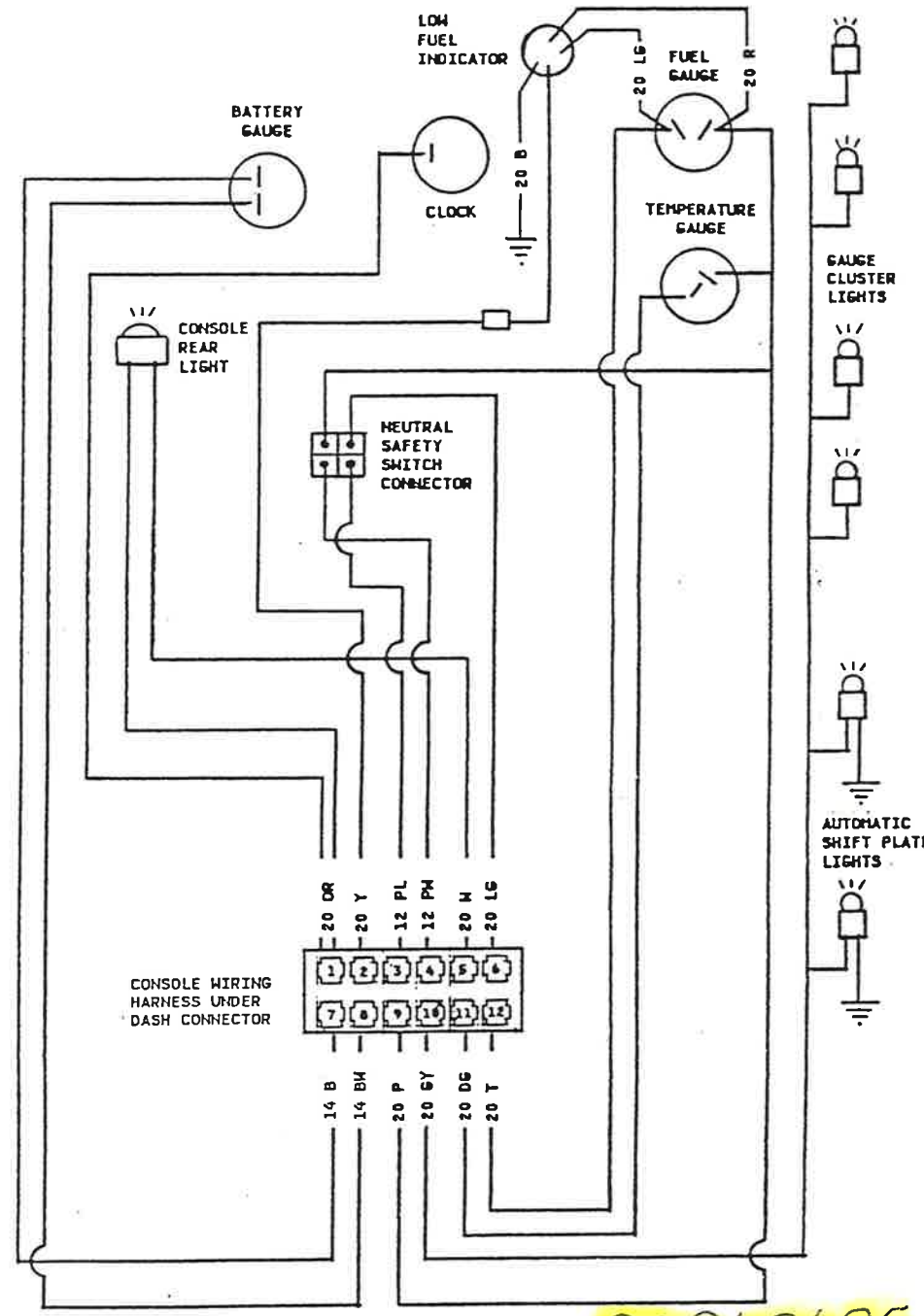
1967 CONSOLE WIRING AUTOMATIC TRANSMISSION WITH CONSOLE GAUGES
